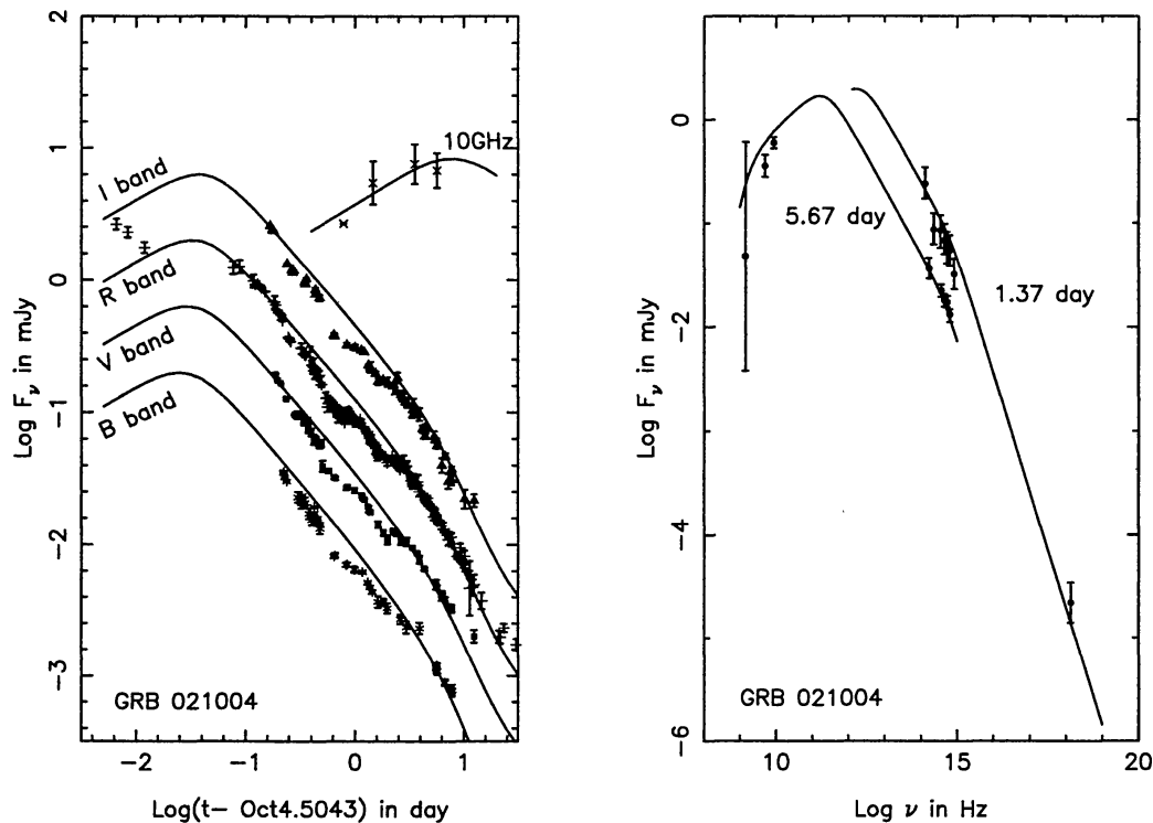
Figure 3. Multi-band observed light curves (left panel) and broadband spectrum (right panel) of the GRB 021004 OA are compared with model predictions shown as solid curves. A total extinction of E(B - V) = 0.20 mag has been used. For clarity of display, in the left panel the B, V, I and radio light curves are shifted vertically by -1.0, -0.5, +0.5 and +1.0 respectively in logarithmic scale. The radio light curve at 10 GHz is constructed, by extrapolation with expected spectral slope, from measurements reported at 22.5 GHz, 15 GHz and 8.46 GHz at different epochs (Frail & Berger 2002, Pooley et al. 2002, Berger et al. 2002). The frequency of 10 GHz was chosen to correspond with a similar plot presented by Kobayashi & Zhang (2003). The model uses \nu_a = 2.1 GHz, \nu_m = 2.5 \times 10^{14} Hz and \nu_c = 3.3 \times 10^{16} Hz at t = 0.06 day; a jet break time t_b = 6.7 day and an electron energy distribution index p = 2.27 . The model includes the host galaxy contribution estimated in section 3.2. In the right panel an expected spectrum with p = 2.27 is shown with the Chandra HETG measurement (Sako & Harrison 2002a) and optical and near-IR observations at the same epoch, \sim 1.37 day. A similar spectrum is also shown at t = 5.67 day, the epoch of the cm-wave radio observations reported by Berger et al. (2002). Where necessary, fluxes measured at optical, near-IR and radio wavelengths were interpolated between adjacent data points at one wavelength in order to determine a contemporaneous value with another wavelength.
