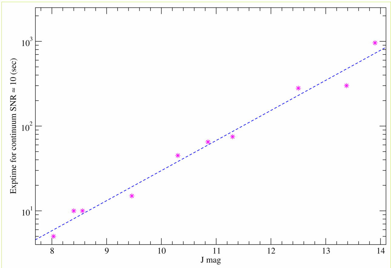
Figure 1: Exposure time for a continuum SNR \sim 10 in the J-band versus J-band magnitude plot for TANSPEC XD-mode observations (Slit 0.5 arcsec).
