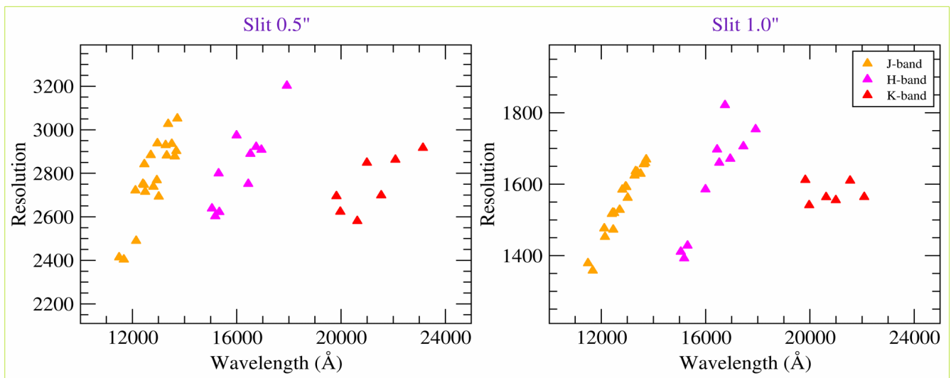
Figure 2: Resolution versus wavelength plot for the slit of width 0.5 arcsec (left) and 1.0 arcsec (right) in XD-mode. Ar-lamp is used for resolution estimation.
